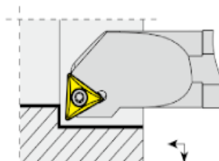
Internal TC.. Holder
