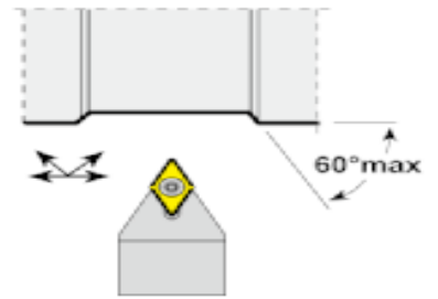
External DC.. Holder
