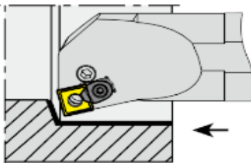
Internal SN.. Holder
