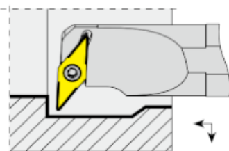
Internal VB.. Holder
