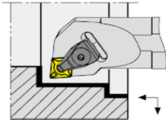
Internal CN.. Holder
