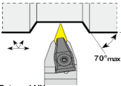
External VN.. Holder
