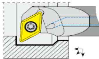
Internal DC.. Holder
