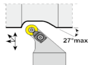
External RC.. Holder
