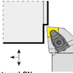
External CN.. Holder
