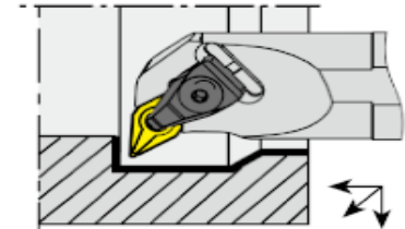
Internal DN.. Holder
