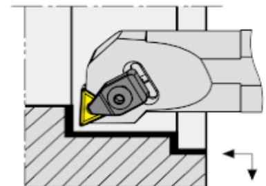
Internal TN.. Holder
