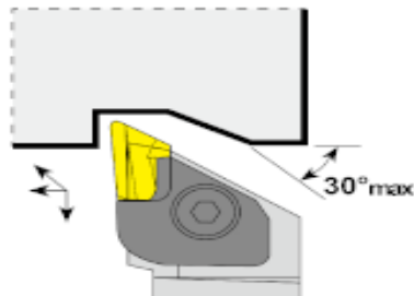
External KN.. Holder
