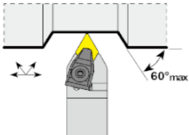
External DN.. Holder
